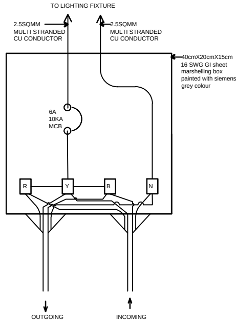
WIRING DIAGRAM OF MARSHALLING BOX
