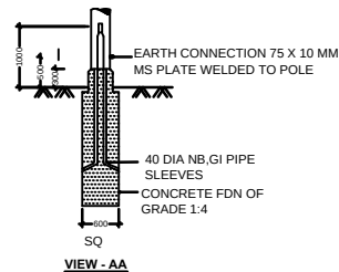
TYPICAL INSTILLATION OF STREET LIGHT POLE
