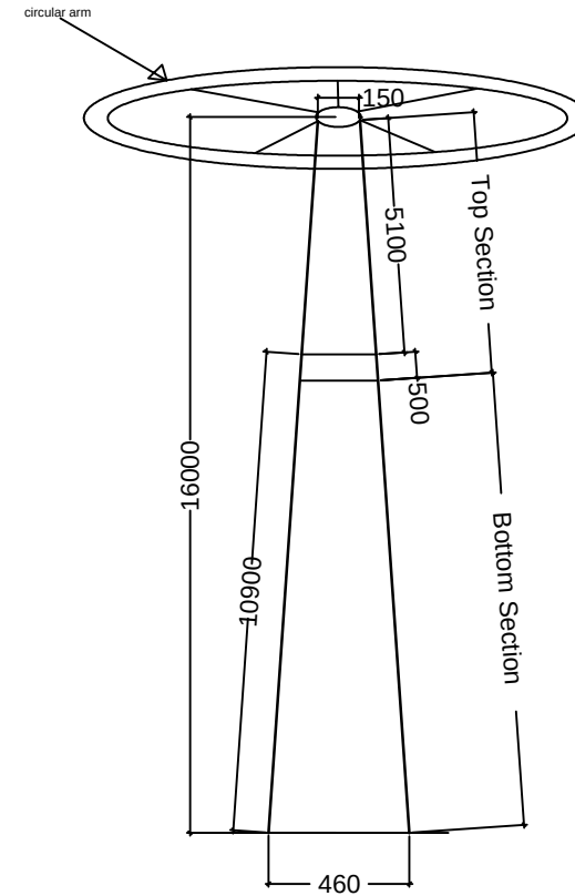
HIGH MAST POLE DIMENSIONS
